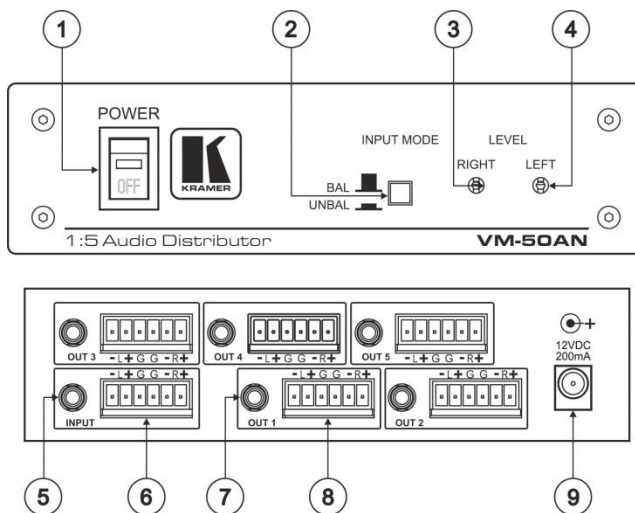
Figure 1: VM-50AN 1:5 Audio Distributor
