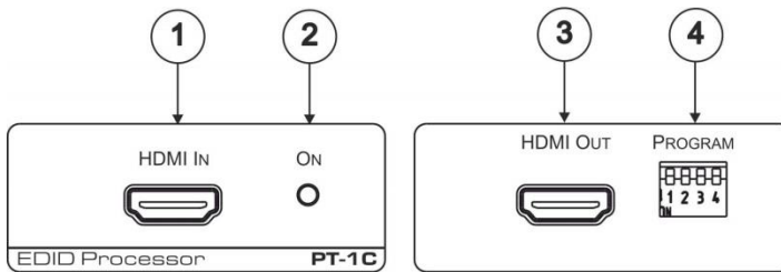
Figure 1: PT-1C EDID Processor
