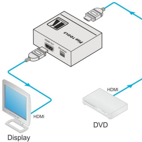
Figure 2: Connecting the PT-1C EDID Processor
