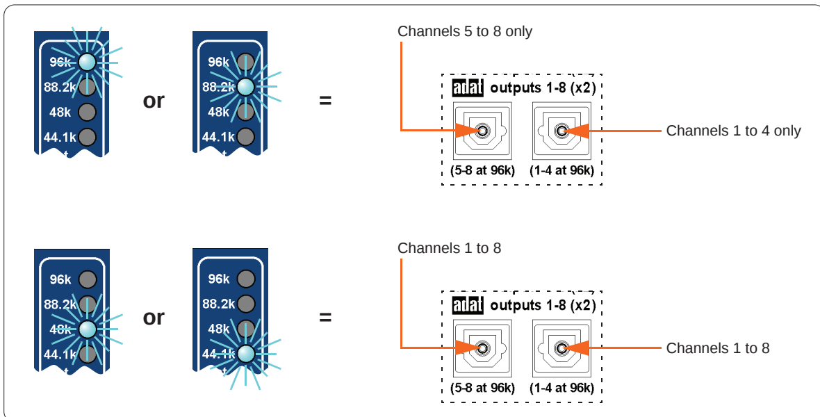
Figure 4: Available ADAT output channels per sample rate.
