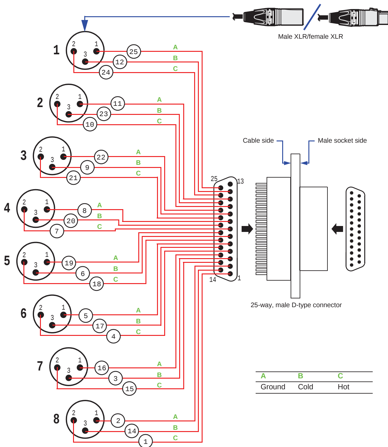
Figure 2: Analogue input (parallel analogue inputs 1-8 connector) and output (analogue outputs 1-8 connector) adapter cable pinouts for a 25-way D-type connector to eight XLRs using the standard "Tascam" pinout configuration. These type of 'off-the-shelf' cables are generally easily obtainable.
