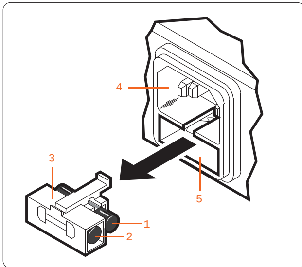
Figure 5: Mains fuse compartment on rear panel.
