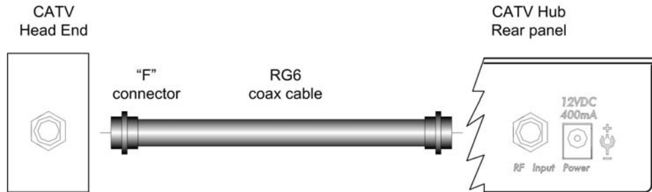
Figure 2: CATV Distribution Hub
