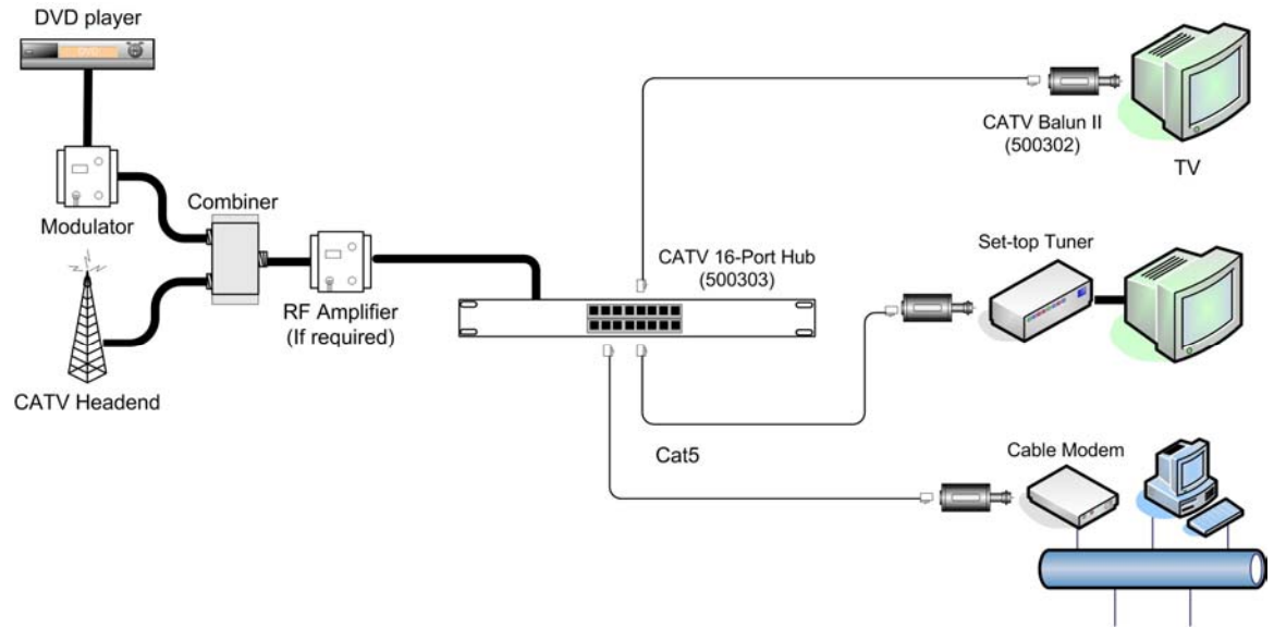
Figure 4: Typical Configuration, CATV & RF Modulation
