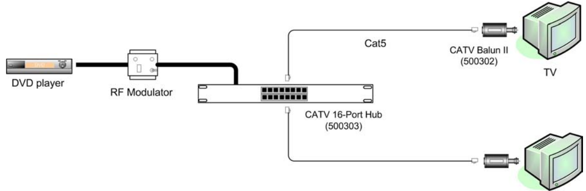
Figure 3: Typical Configuration, RF Modulation
