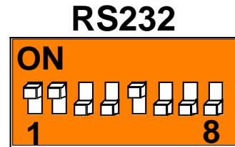
Figure 10- RS232 DIP switches
