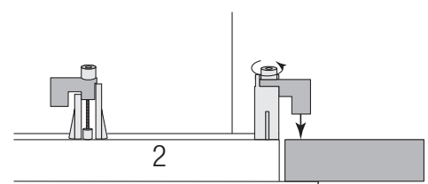
Dog-ears against loudspeaker
