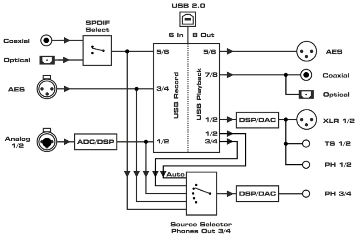
ADI-2 Pro USB Mode, 6/8 channels
