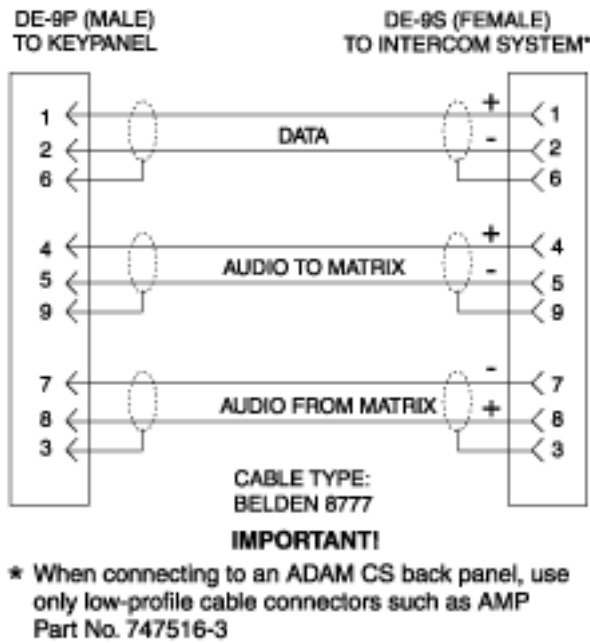
FIGURE 8. DE9 Intercom Cable
