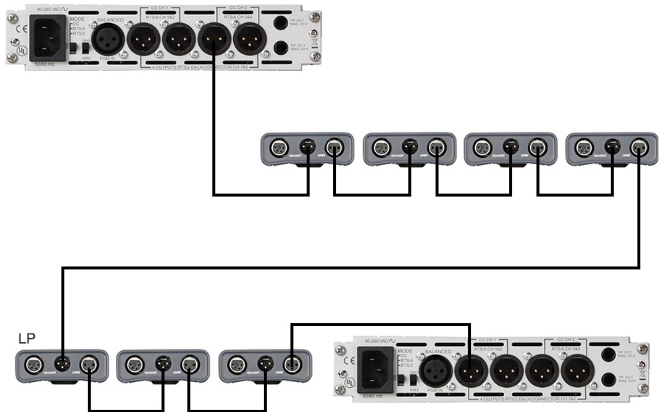
FIGURE 3. Two Power Supply System
