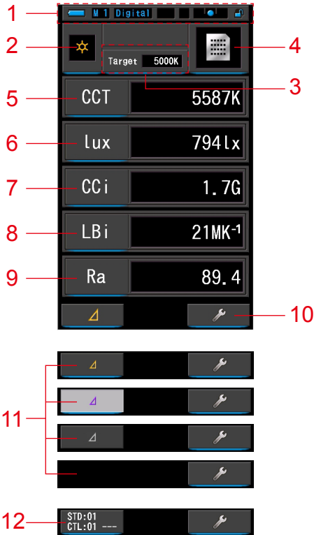
Measuring Screen in Text Mode
