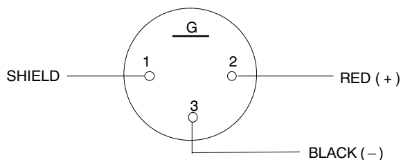
A400XLR CONNECTOR TERMINALS
