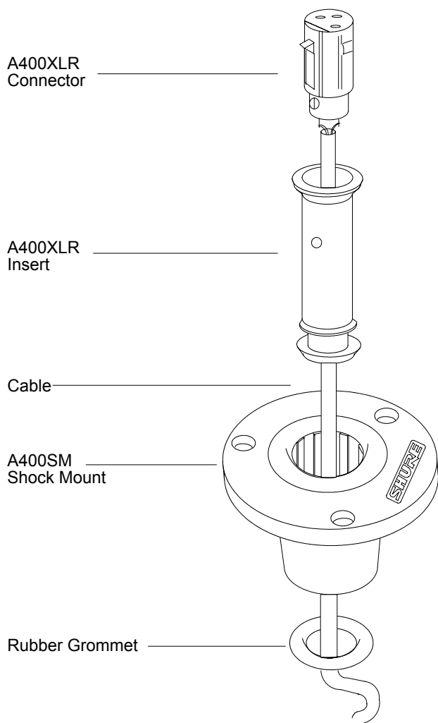
COMPONENTS OF THE A400SMXLR FIGURE 1
