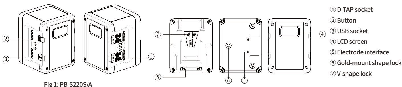
Fig 1: PB-S220S/A
