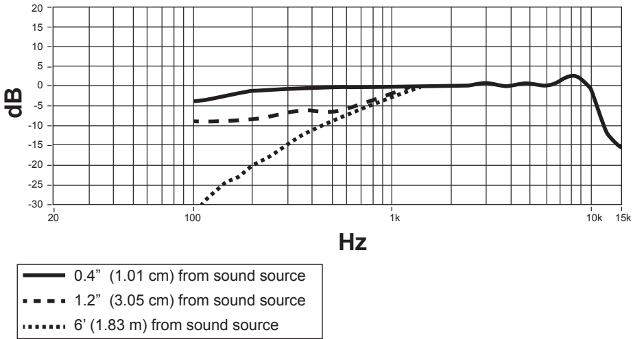
Frequency Response
