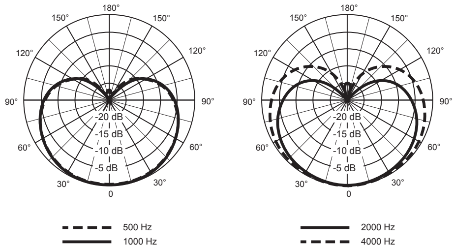
Polar Pattern
