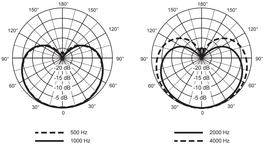
Polar Pattern
