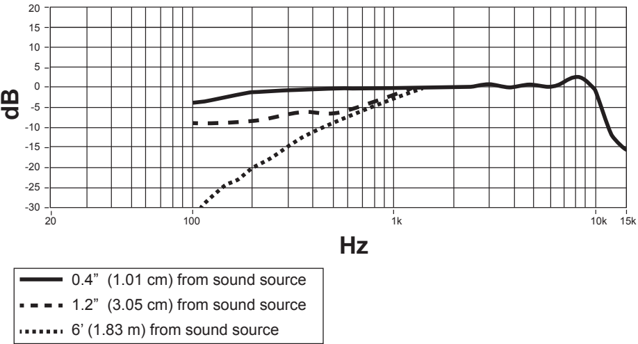
Frequency Response
