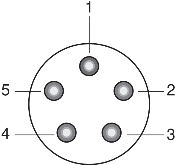
Cable 5-pin connector (male)
