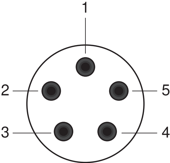
Bodypack 5-pin connector (female)
