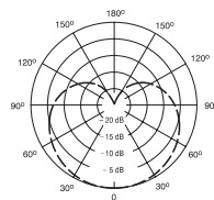
Typical Polar Pattern
