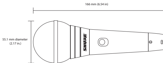
Overall Dimensions
