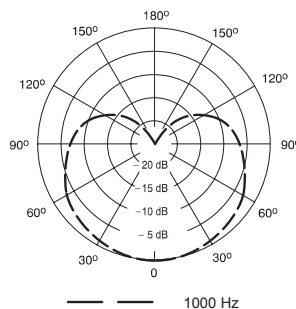
Polar Pattern
