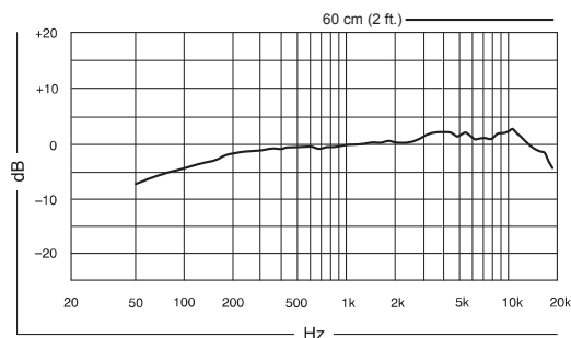
Frequency Response
