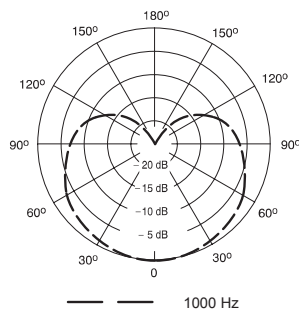
Polar Pattern
