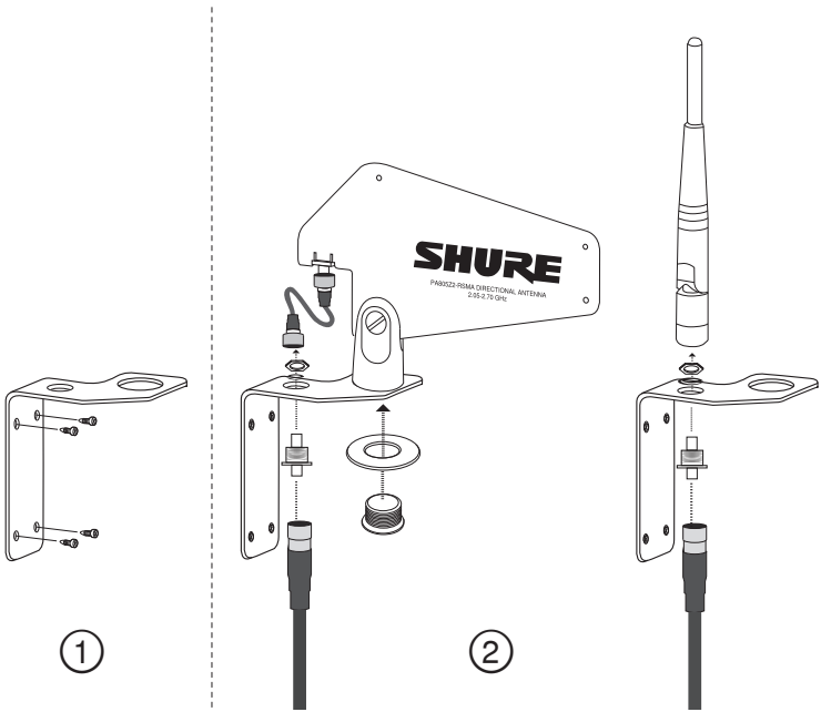
Wall Mount
