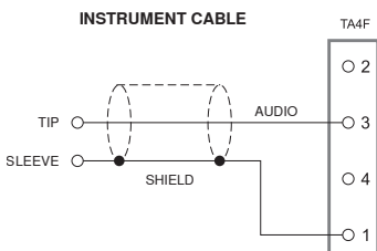
INSTRUMENT CABLE
