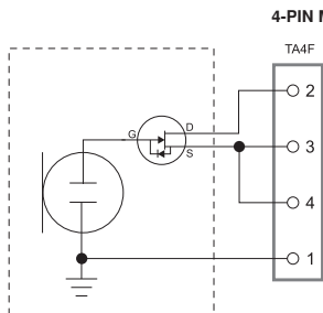
CONDENSER MICROPHONE
