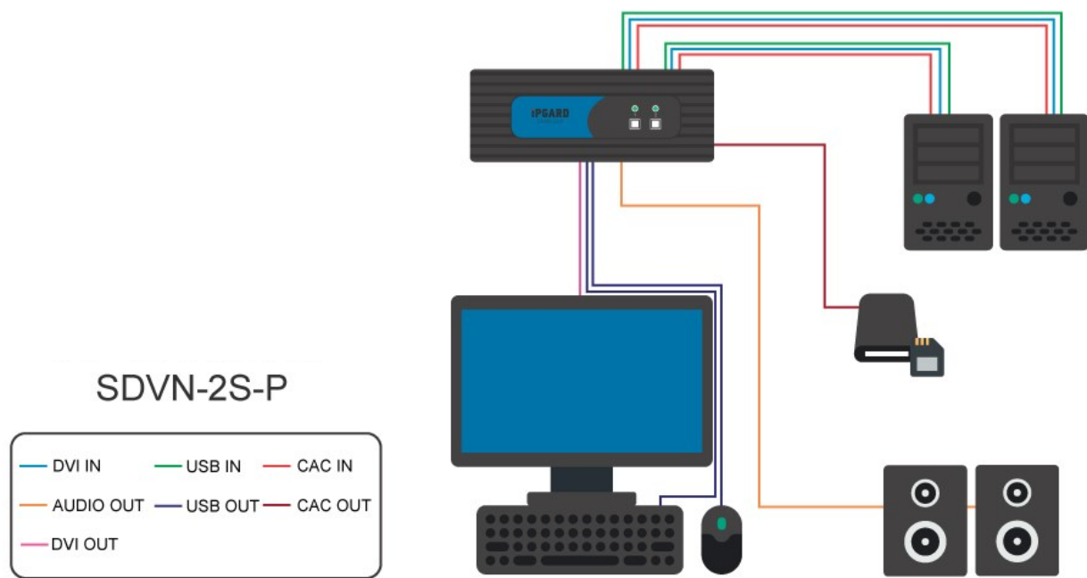
Figure 8-2 SDVN-2S-P Shown
