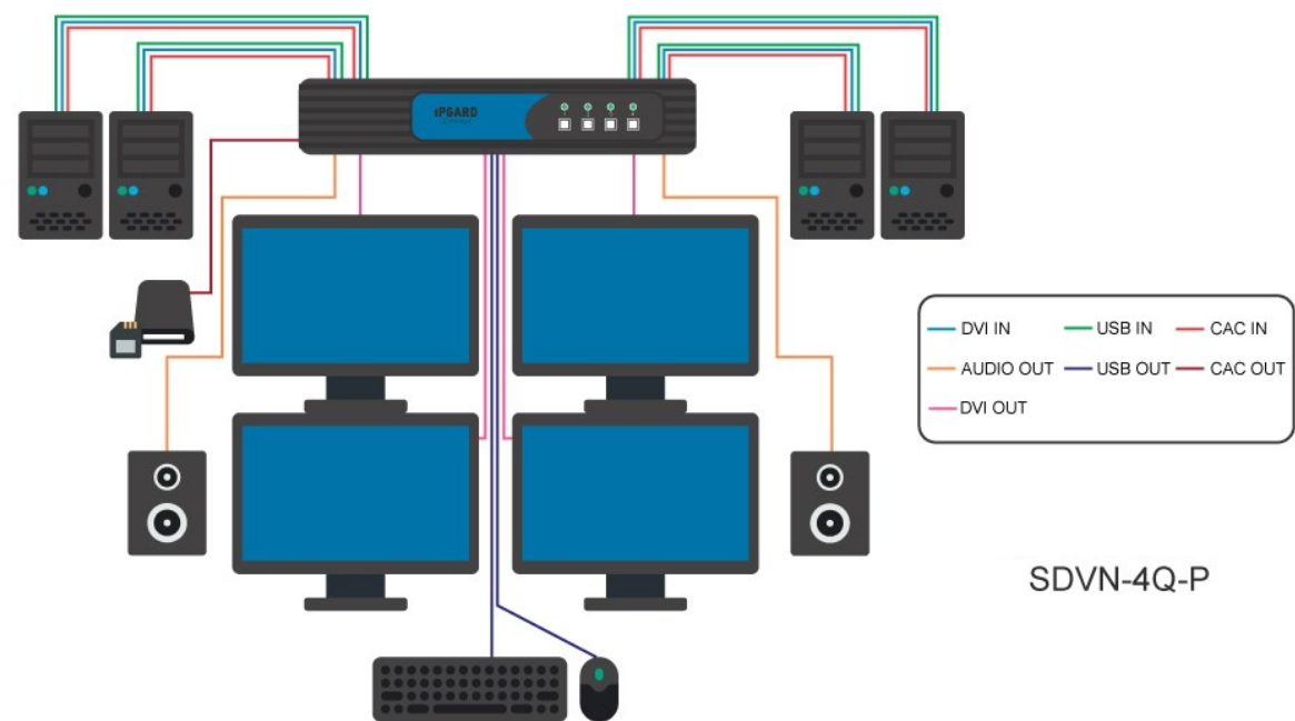
Figure 8-1 SDVN-4Q-P Shown
