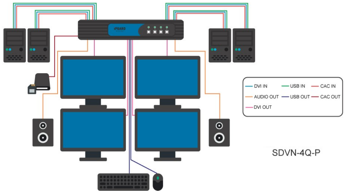
Figure 8-1 SDVN-4Q-P Shown
