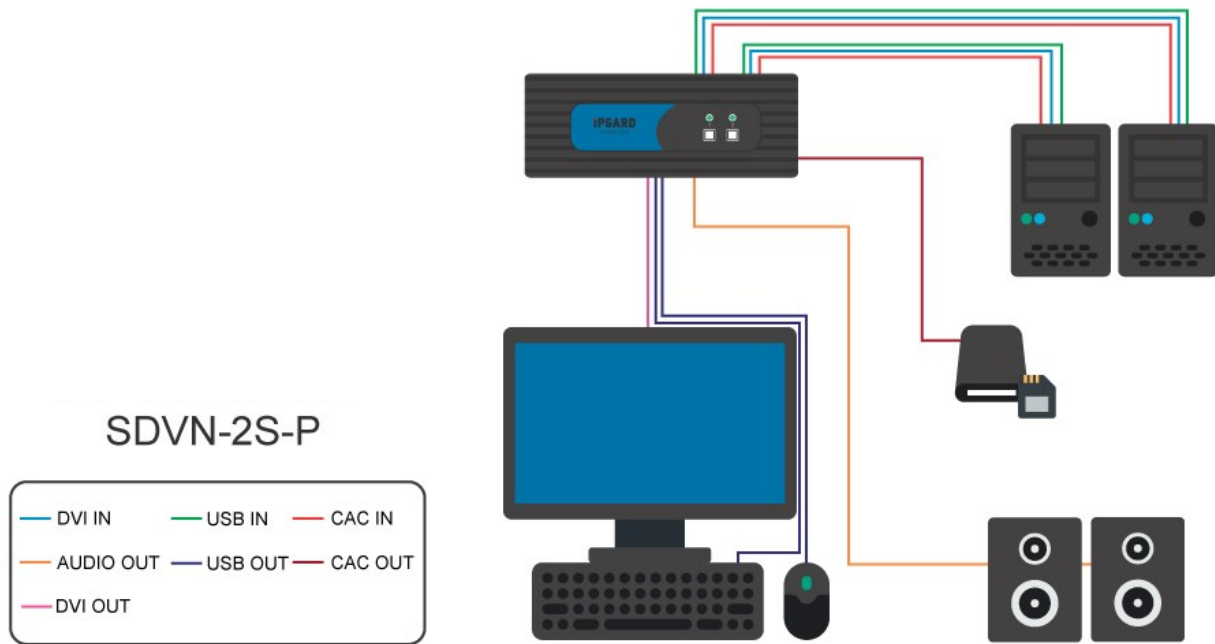
Figure 8-2 SDVN-2S-P Shown
