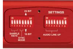
Fig 1-7: DIPSwitch Settings
