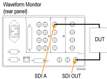
Figure 17: Signal generation connection
