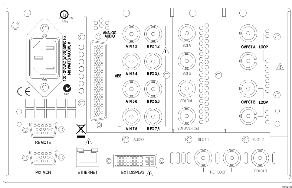
Figure 2: Rear panel
