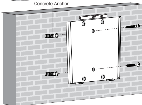
Concrete Anchor
