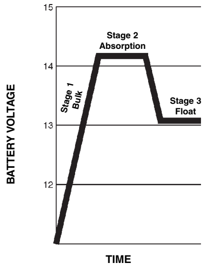
CHARGING PROFILE
