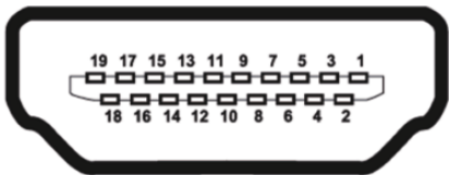
Type A (Receptacle) HDMI
