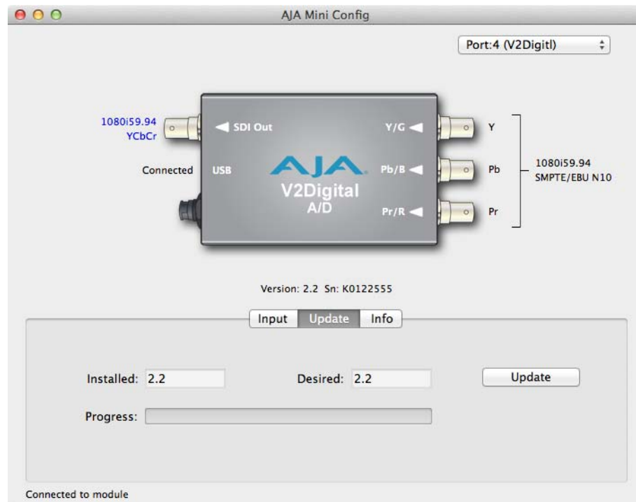
Figure 8. MiniConfig, Update Screen
