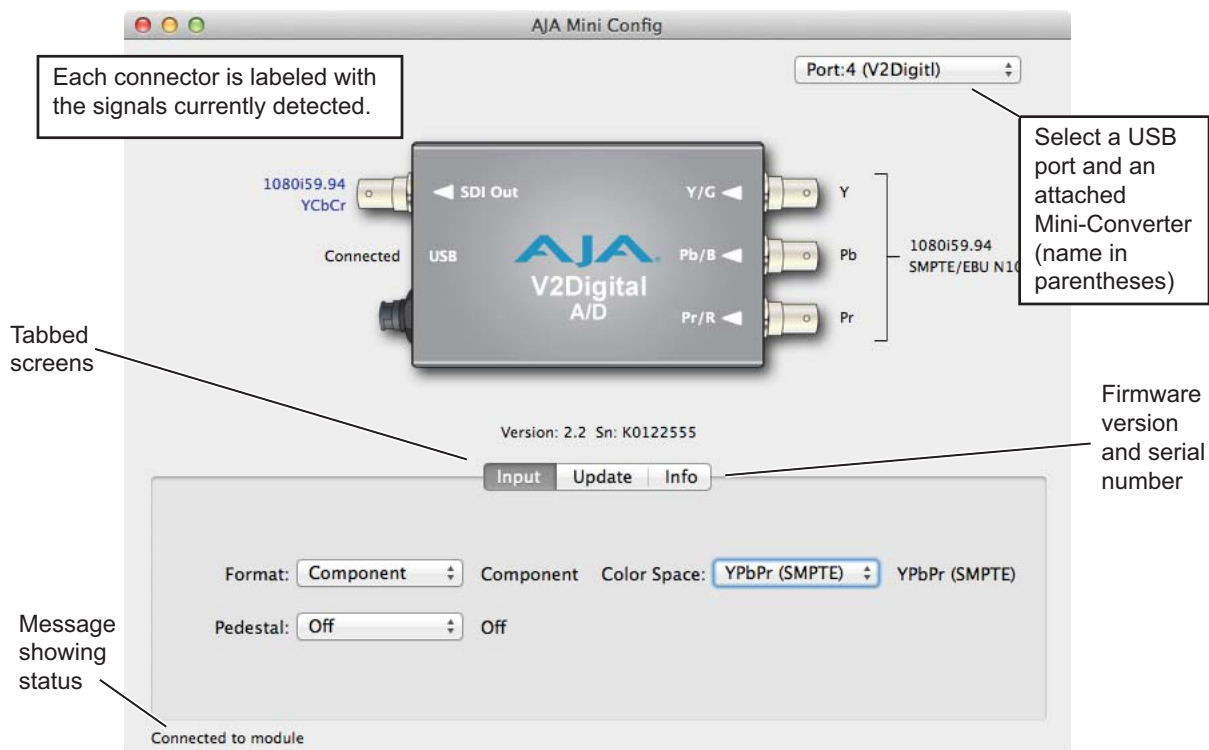
Figure 6. MiniConfig Screen
