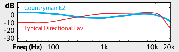
Countryman E2 and typical cardioid lavalier on the chest, approximately gain matched for the voice band at the mix board.
