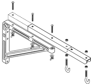
No. 23 Adjustable Wall Bracket Screen can be extended 10", 14", 15¾", 18¾", 20" or 24" from wall by wing nut and bolt adjustment.
