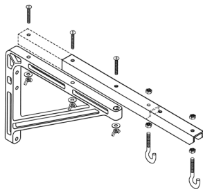
No. 23 Adjustable Wall Bracket Screen can be extended 10", 14", 15¾", 18¼", 20" or 24" from wall by wing nut and bolt adjustment.
