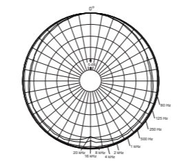
Polar Pattern (normalized, SC4071 & SCO71-H)
