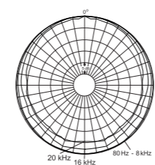
Polar Pattern (normalized, SC4071 & SCO71-H)
