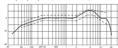
Frequency Response (SC4071 & SCO71-H)
