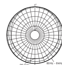
Polar Pattern (normalized, SC4071 & SCO71-H)
