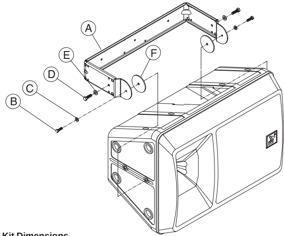
FIGURE 2 — Mb200 Installation Kit Dimensions
