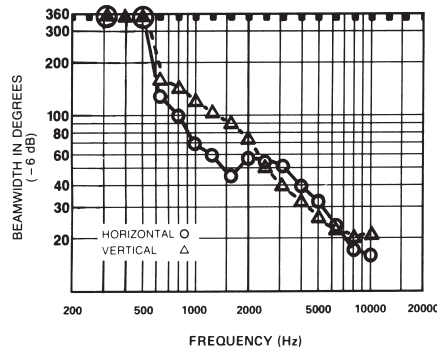
Figure 2 CFID32 Beamwidth vs. Frequency
