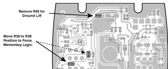
Figure 3: PCB Jumper Locations
