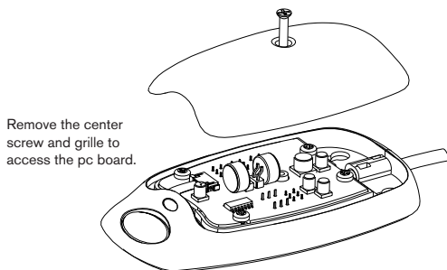
Figure 2: PCB Access
