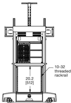
rear view
