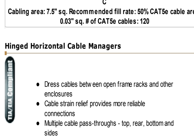
C Cabling area: 7.5" sq. Recommended fill rate: 50% CAT5e cable area: 0.03" sq. # of CAT5e cables: 120
