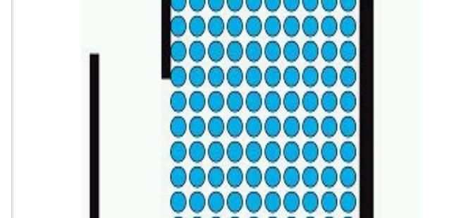
A Cabling area: 0.45" sq. Recommended fill rate: 50% CAT5e cable area: 0.03" sq. # of CAT5e cables: 7
