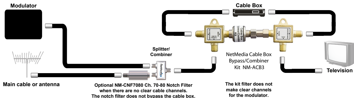
Figure 4 - Bypassing a digital or analog cable box and recombining to a single coax input on the TV. The kit's filter removes any conflict on channel 3 or 4. Switch TV from the cable box to the modulator channel.
