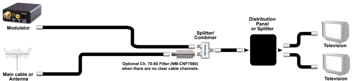
Figure 2 - Connecting the modulator to an antenna or cable service and distributing to multiple televisions.
