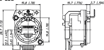
NE8FBH-C5-LED
