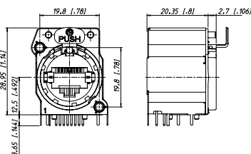
NE8FBV-C5-LED-S
