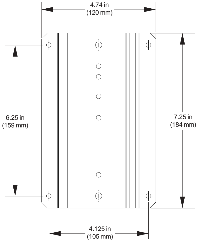
FRONT VIEW (WALL PLATE DETAIL)
