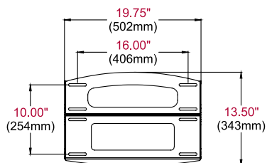
WALL PLATE
