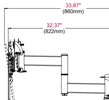
SIDE VIEW EXTENDED +10°/-5° TILT
