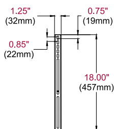
ADAPTOR BRACKET
