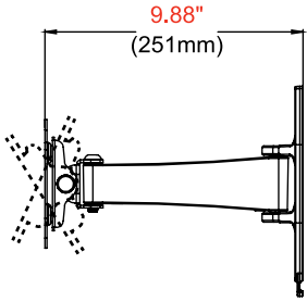
SIDE VIEW EXTENDED +/-35° TILT
