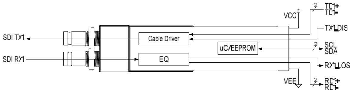
Block Diagram
