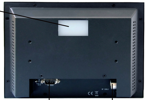
VF-PBM-209 Back / Connections
