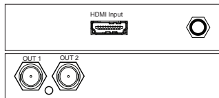
PRO-HDMI2HD HDMI INPUT TO 3G/HD/SDI OUTPUT
