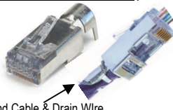
External Ground Around Cable & Drain Wire
